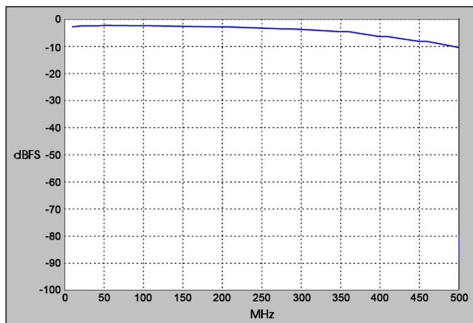
Input Frequency Response
