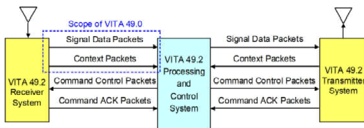
Figure 2. VITA 49.2 supports transmitter Signal Data Packets plus command and control functions
