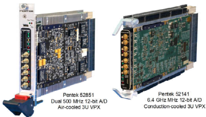
Figure 3. 3U VPX software radio modules include FPGA-based VITA 49 protocol engines
