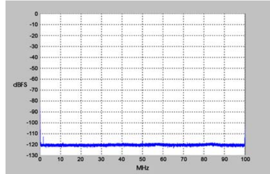
Spurious Pick-up
