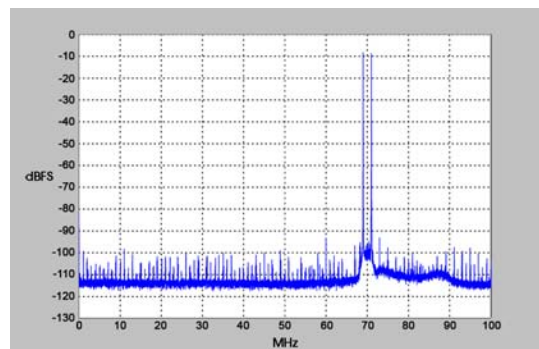
Two-Tone SFDR
